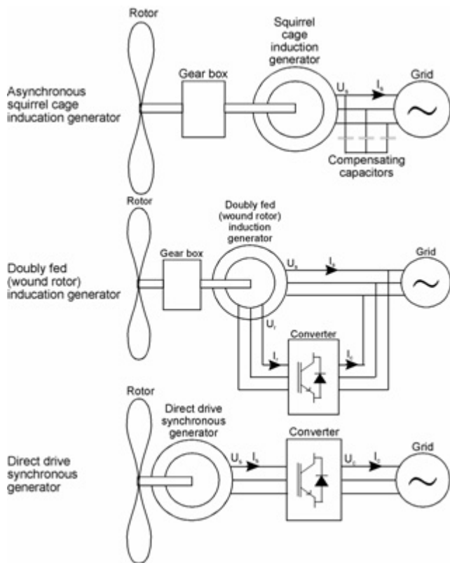
Fig. 4. The three commonly used generator systems.
