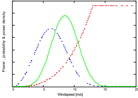
Fig. 3. Power P (red, dashed), probability density U (blue, dotted) and power density (green, solid) as a function of wind speed (arbitrary units)
