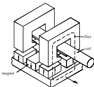
Fig. 6. Transverse flux permanent-magnet generator.
