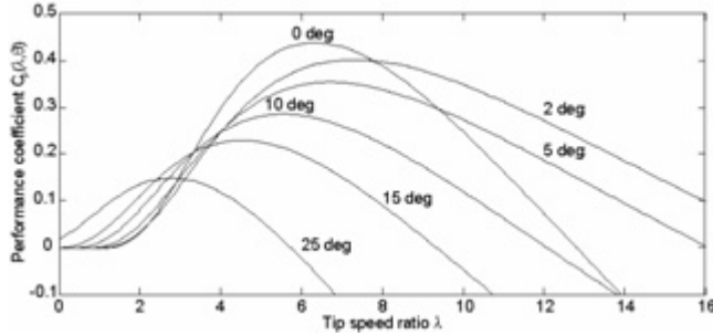
Fig. 2. Power coefficient C_p as a function of tip speed ratio \lambda and pitch angle \theta for a specific blade [3].
