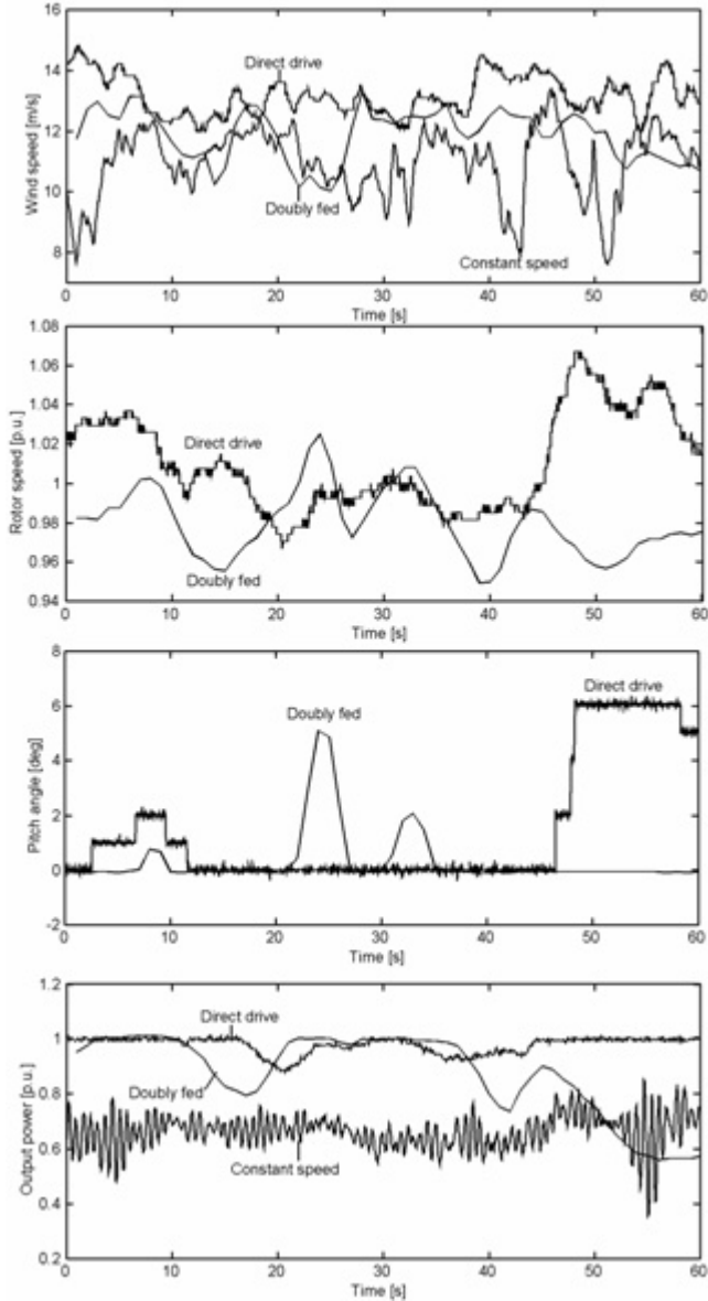
Fig. 5. Measured wind speeds and resulting rotor speeds, pitch angles and output powers for the three different generator systems.
